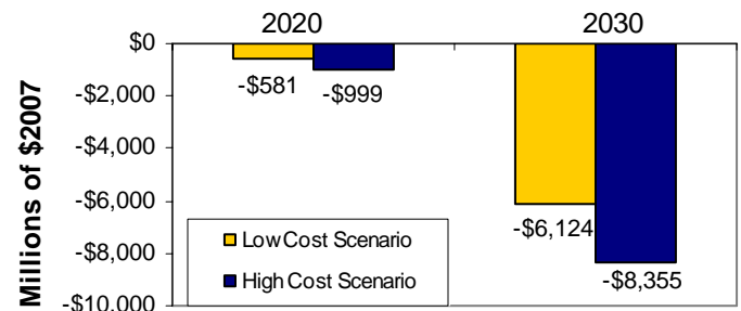
Figure 4. Loss in Gross State Product For Connecticut
